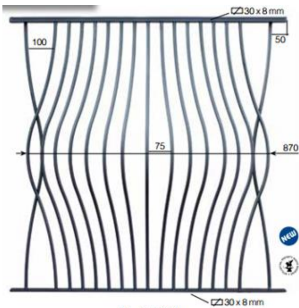
Art. GD288/1 ∅ 12 mm L 1000 mm H 1000 mm
