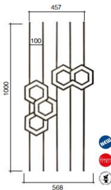
Art. GD301/3 \square 12 x 12 mm 568 x 1000 mm
