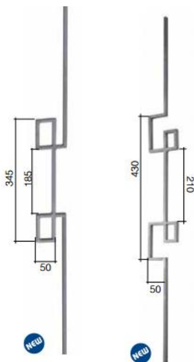
Art. GD202/6 □ 14 x 8 mm L 80 mm H 1000 mm
