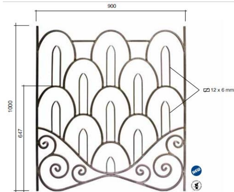
Art. GD291/1 □ 12 x 12 mm + □ 12 x 6 mm L 900 mm H 1000 mm
